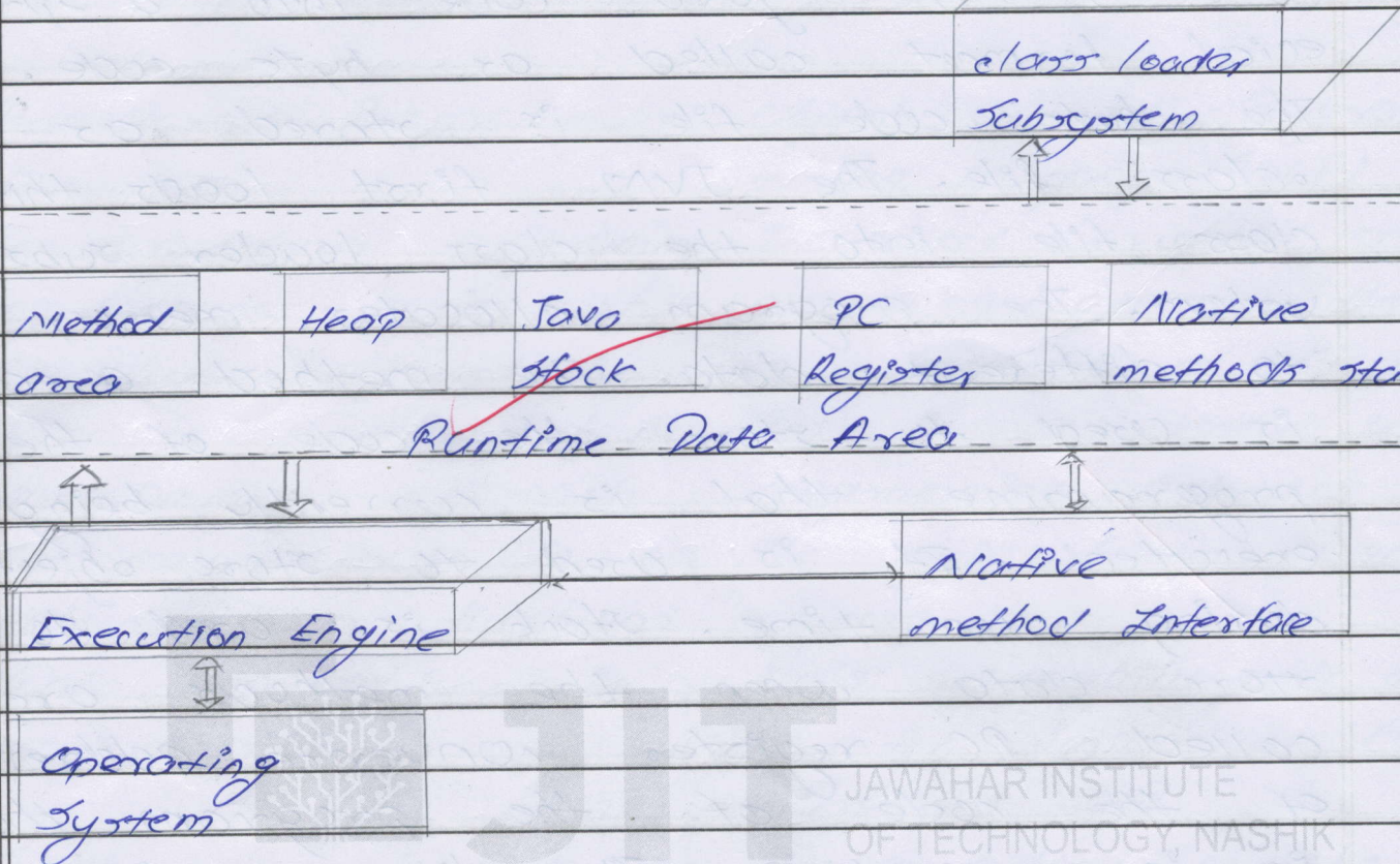
Fig : Java Virtual Machine
